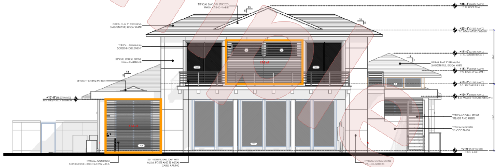
WEST ELEVATION
